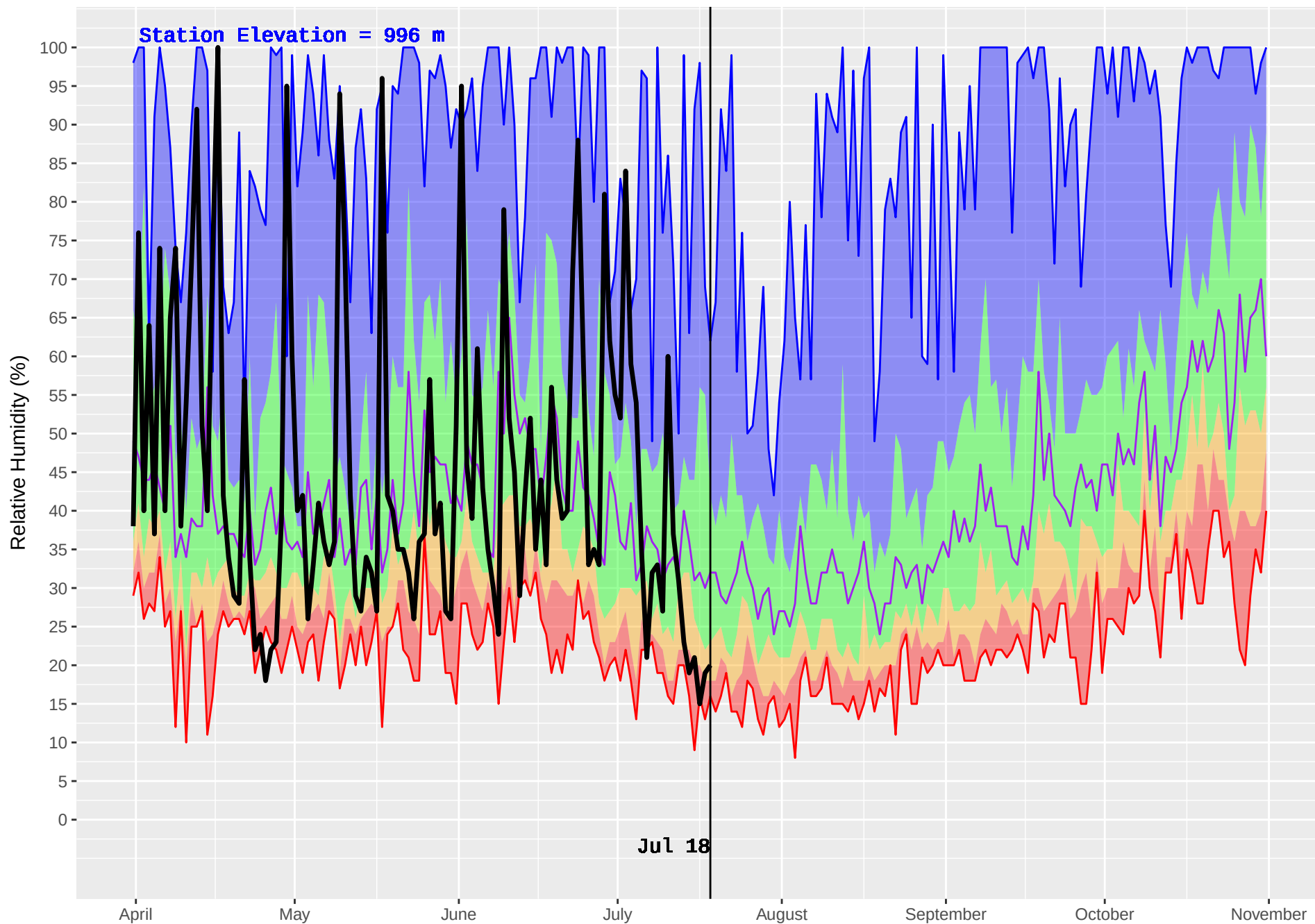
CRANBROOK FS (426) : Historical (2001–2016) and Current (2018) Daily Relative Humidity
