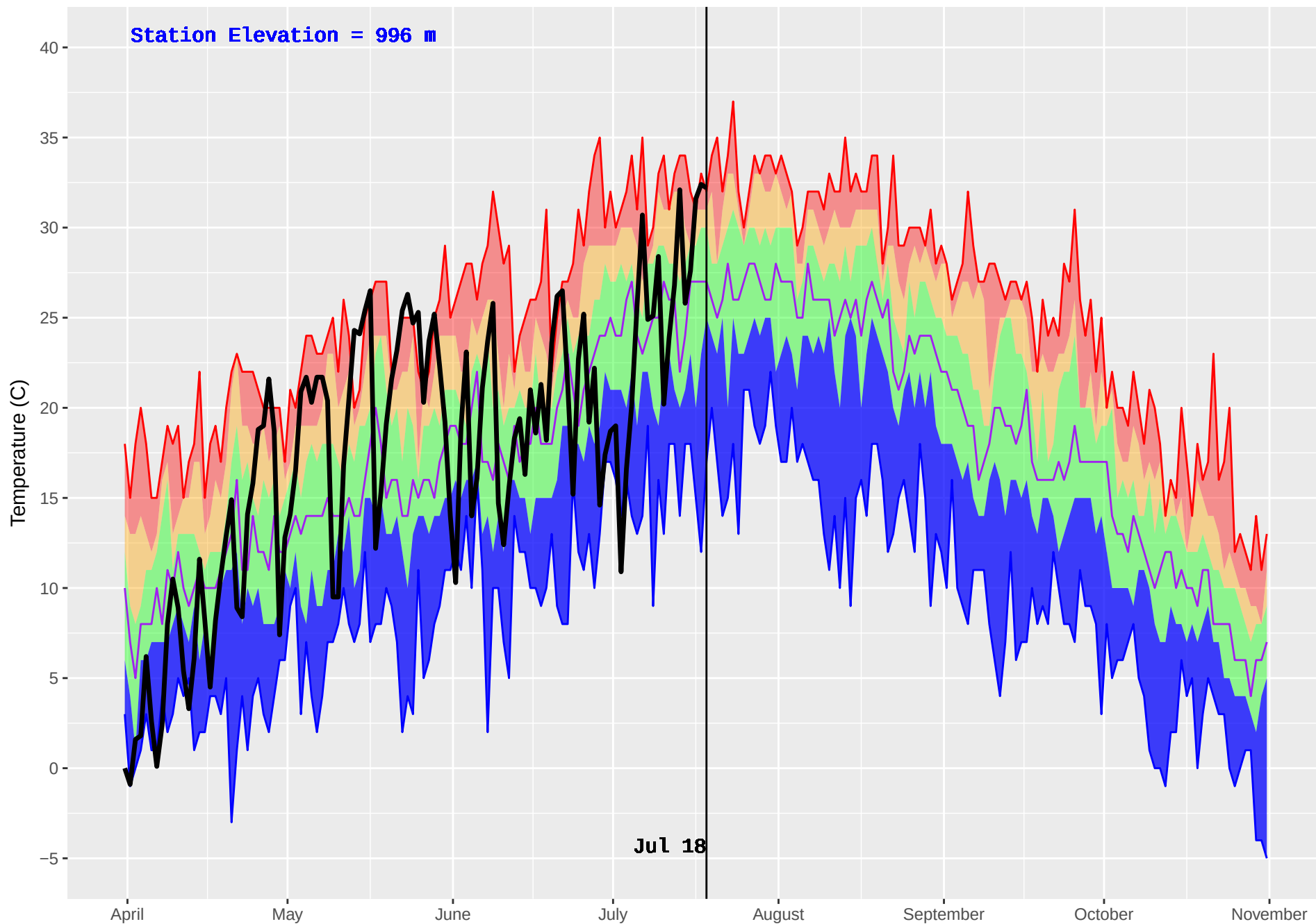
CRANBROOK FS (426) : Historical (2001–2016) and Current (2018) Daily Temperature
